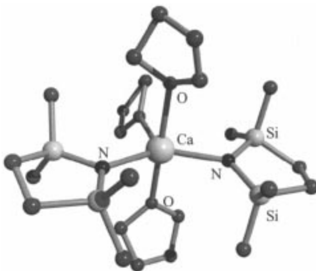
Fig. 5. Molecular structure of tris(tetrahydrofuran)calcium bis[2,2,5,5-tetramethyl-2,5-disilazacyclopentanide]. Hydrogen atoms are omitted for clarity.
