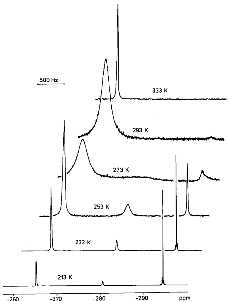
Fig. 11. Dynamic ^{31}\text{P}\{^1\text{H}\} -NMR spectra of tris(1,2-dimethoxyethane- O,O' )barium bis[2,2,5,5-tetramethyl-2,5-disilaphospha-cyclo-pentanide] in toluene- d_8 . Temperatures are given on each spectrum.
