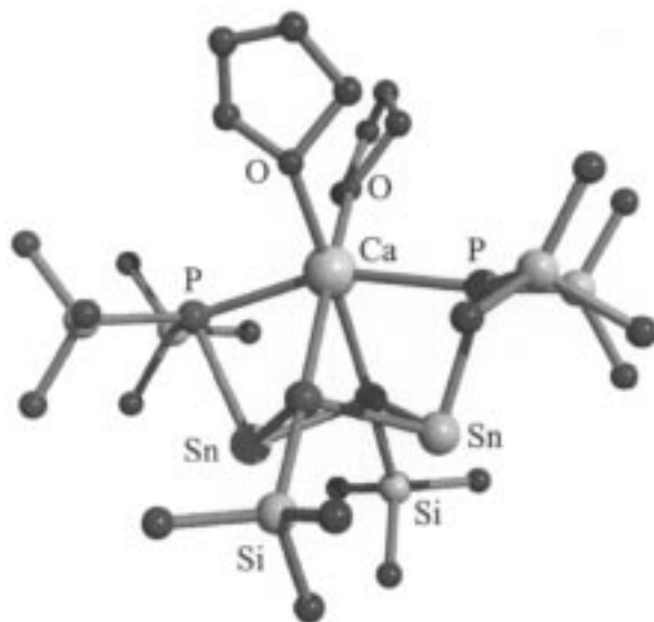
Fig. 14. Molecular structure of the heterobimetallic complex (\text{THF})_2\text{CaSn}_2[\mu_2\text{-P}(\text{SiMe}_3)_2]_2[\mu_3\text{P}(\text{SiMe}_3)_2] . Hydrogen atoms are omitted for clarity.
